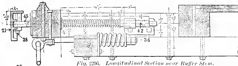
Fig. 2296. Longitudinal Section near Buffer Stem.
